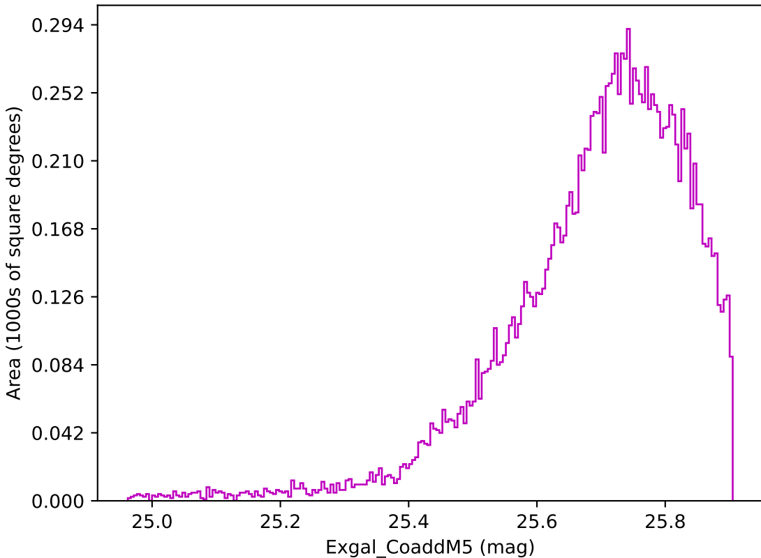
weather_cloudso0v3.4_10yrs WFD z band: Exgal_CoaddM5
