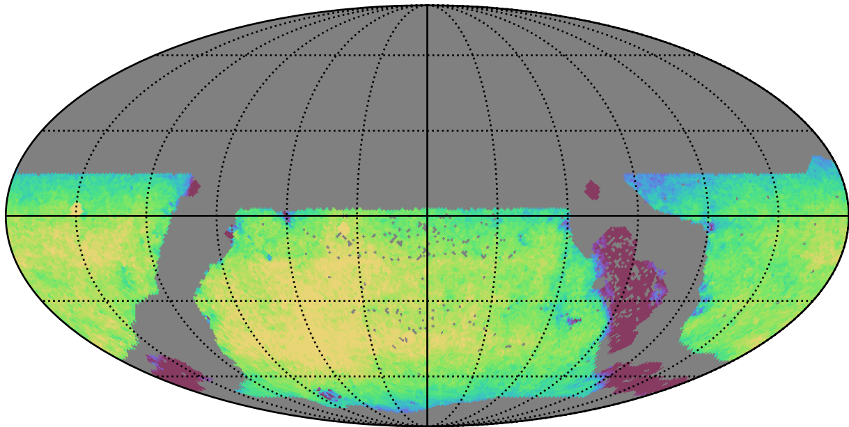
weather_cloudso0v3.4_10yrs WFD y band: Exgal_CoaddM5
