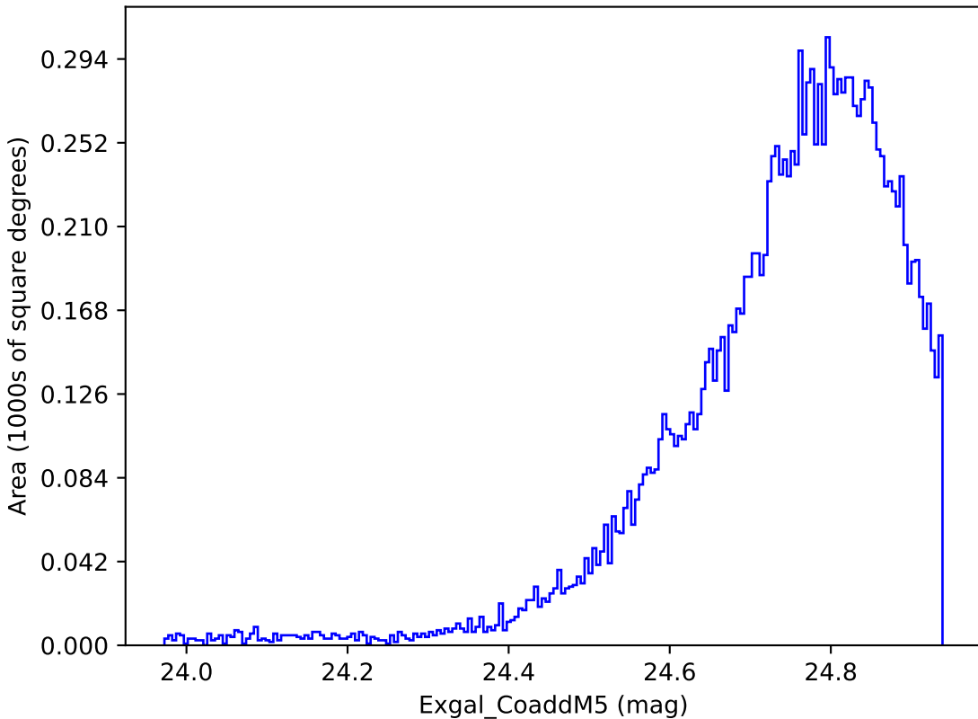
weather_cloudso0v3.4_10yrs WFD y band: Exgal_CoaddM5
