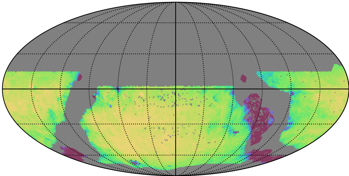
weather_cloudso0v3.4_10yrs WFD u band: Exgal_CoaddM5
