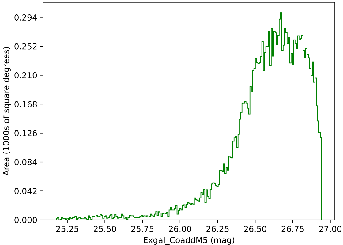
weather_cloudso0v3.4_10yrs WFD g band: Exgal_CoaddM5
