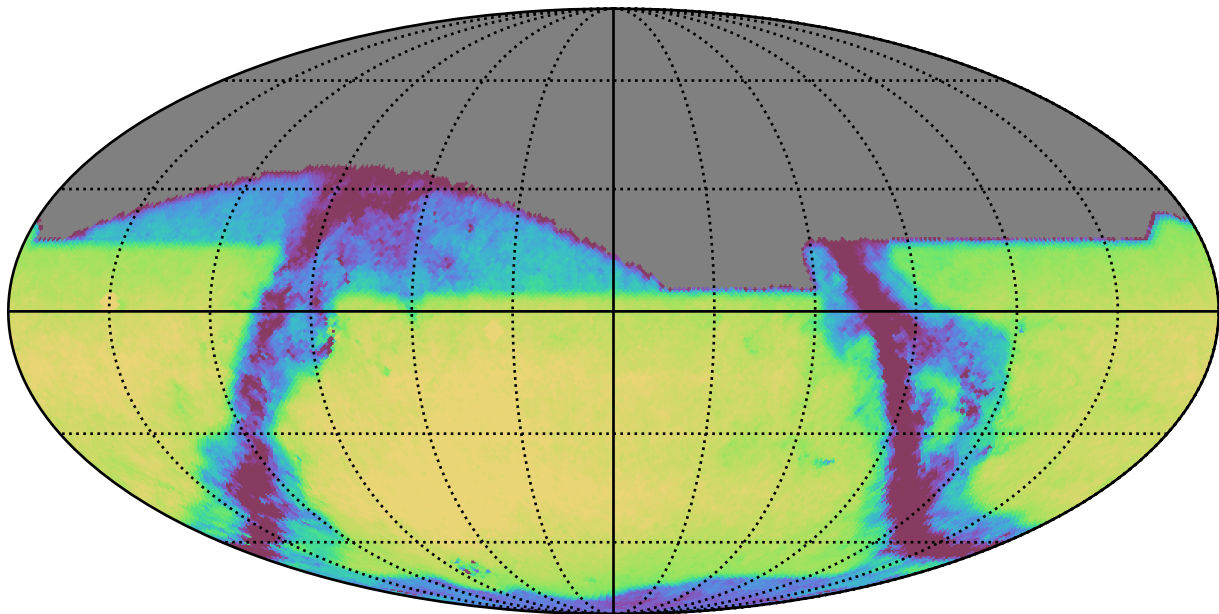
weather_cloudso0v3.4_10yrs All sky z band: Exgal_CoaddM5
