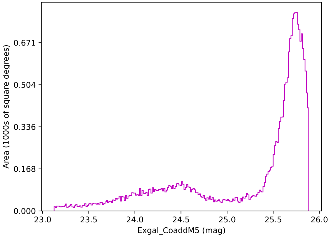
weather_cloudso0v3.4_10yrs All sky z band: Exgal_CoaddM5
