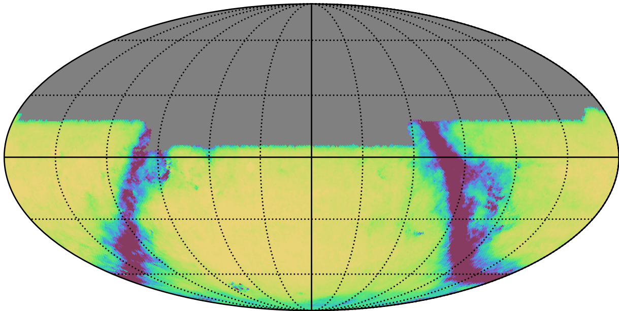
weather_cloudso0v3.4_10yrs All sky u band: Exgal_CoaddM5
