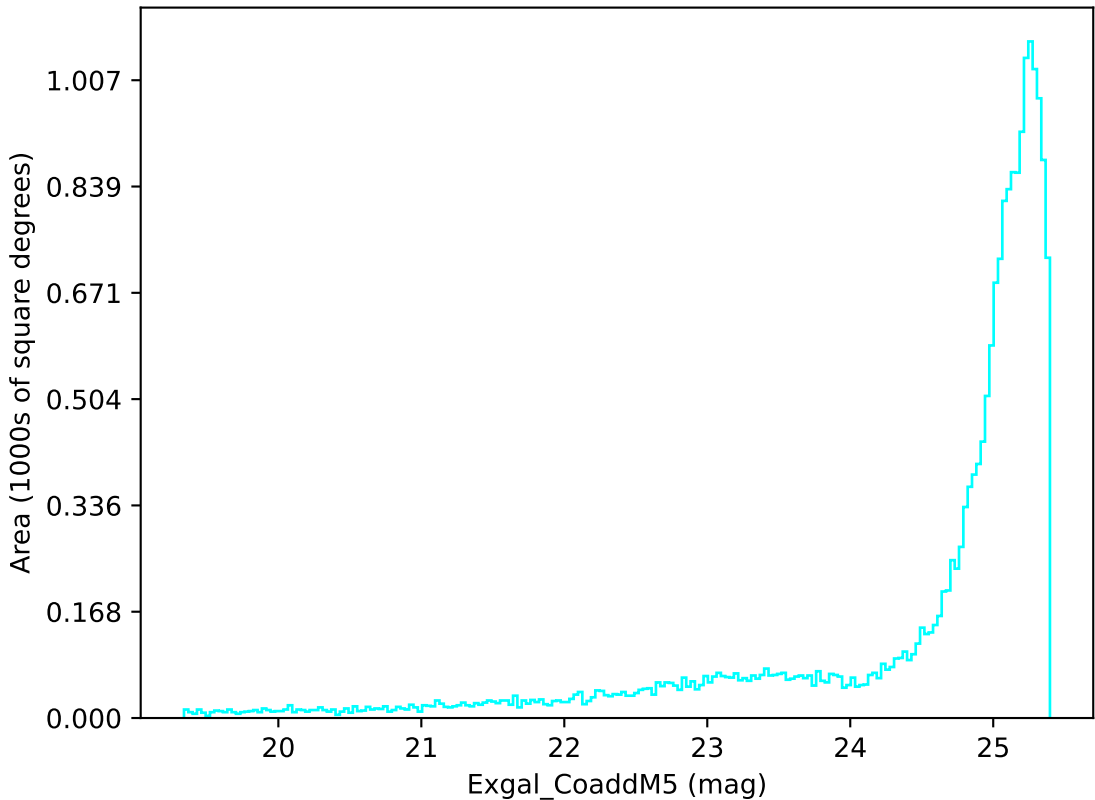
weather_cloudso0v3.4_10yrs All sky u band: Exgal_CoaddM5
