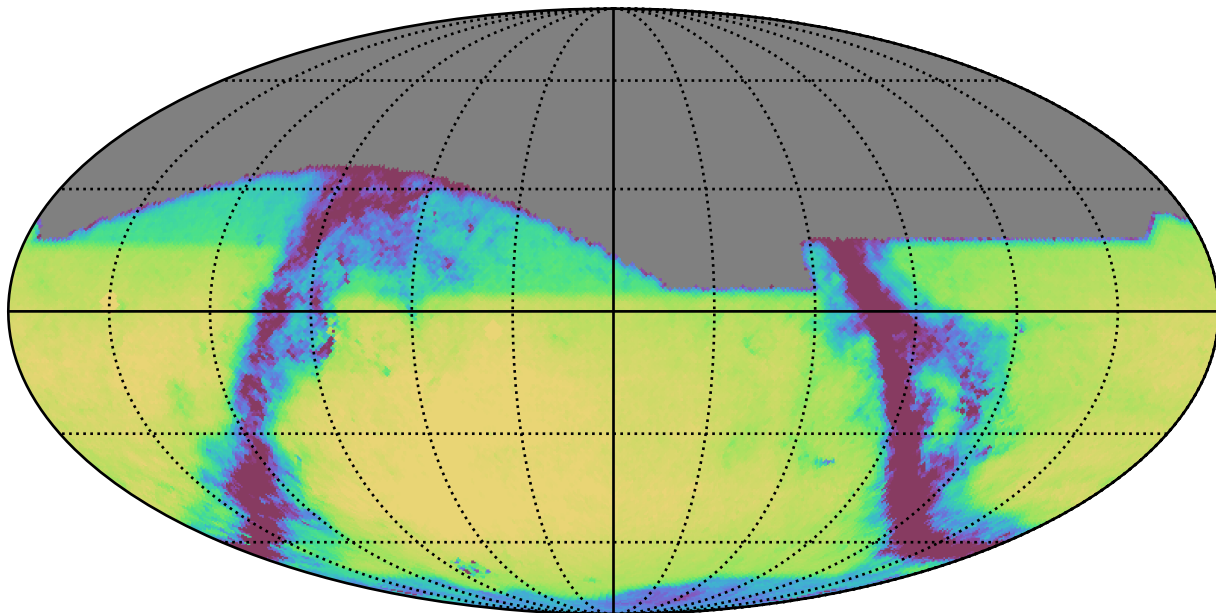
weather_cloudso0v3.4_10yrs All sky r band: Exgal_CoaddM5
