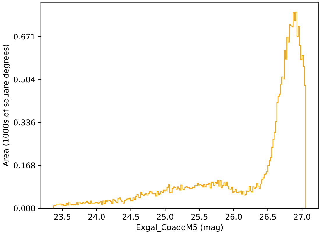
weather_cloudso0v3.4_10yrs All sky r band: Exgal_CoaddM5
