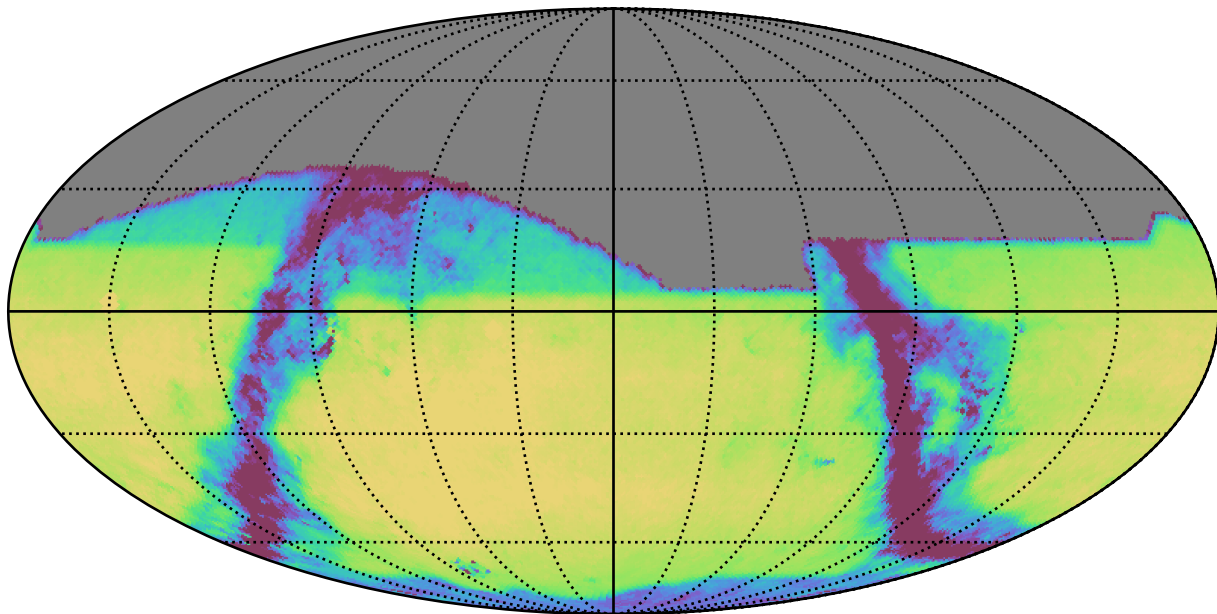
weather_cloudso0v3.4_10yrs All sky i band: Exgal_CoaddM5
