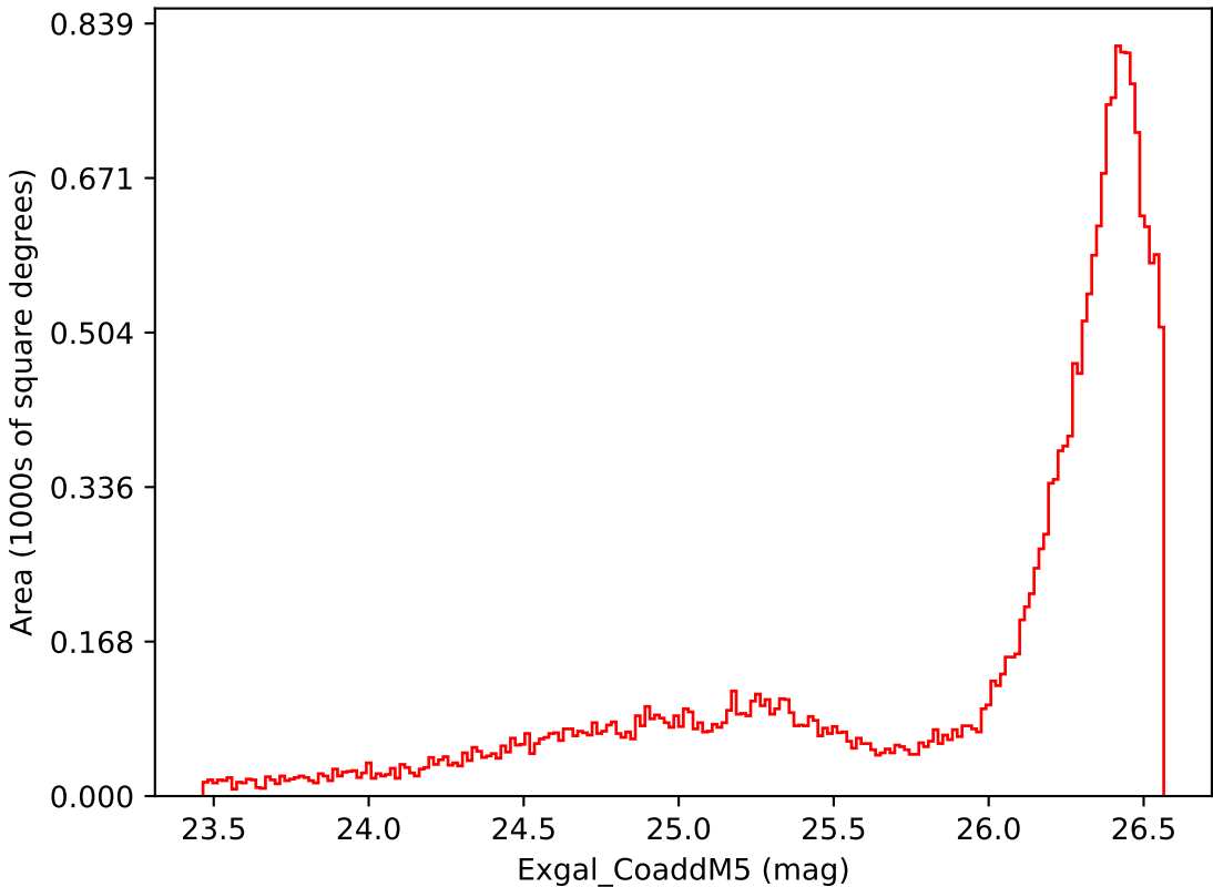
weather_cloudso0v3.4_10yrs All sky i band: Exgal_CoaddM5
