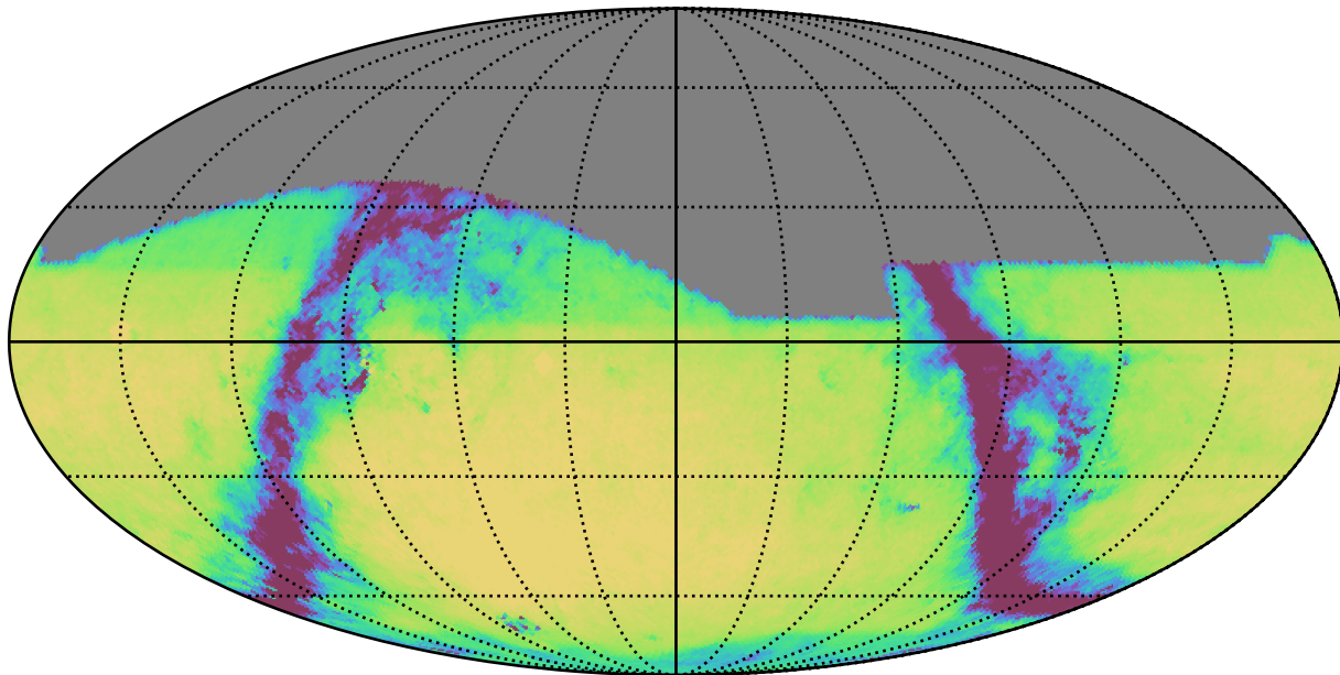
weather_cloudso0v3.4_10yrs All sky g band: Exgal_CoaddM5
