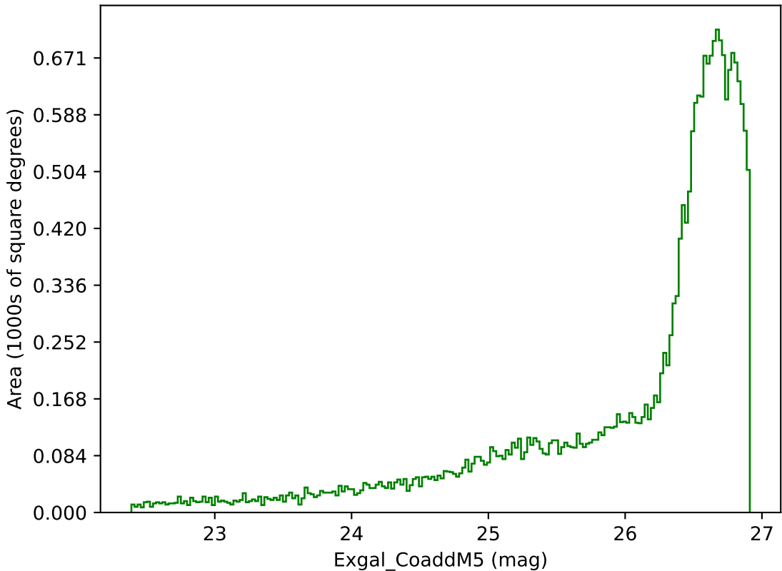
weather_cloudso0v3.4_10yrs All sky g band: Exgal_CoaddM5
