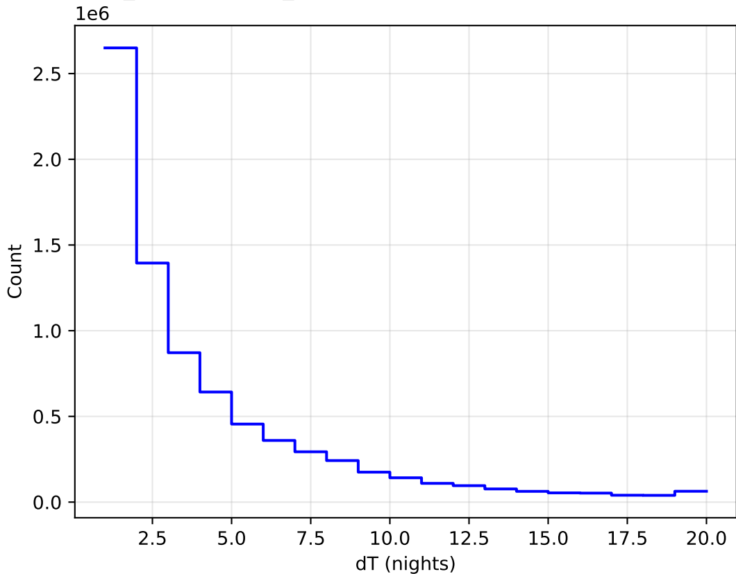
weather_cloudso0v3.4_10yrs WFD all bands: DeltaNight Histogram
