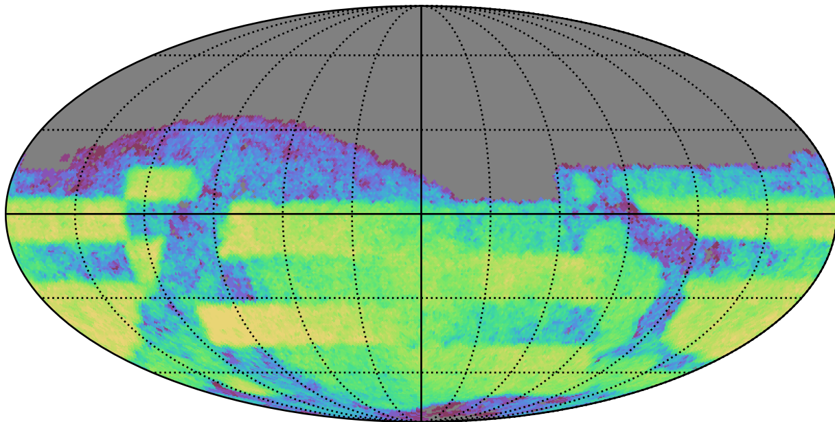
weather_cloudso0v3.4_10yrs Yr 3-4 z band: CoaddM5
