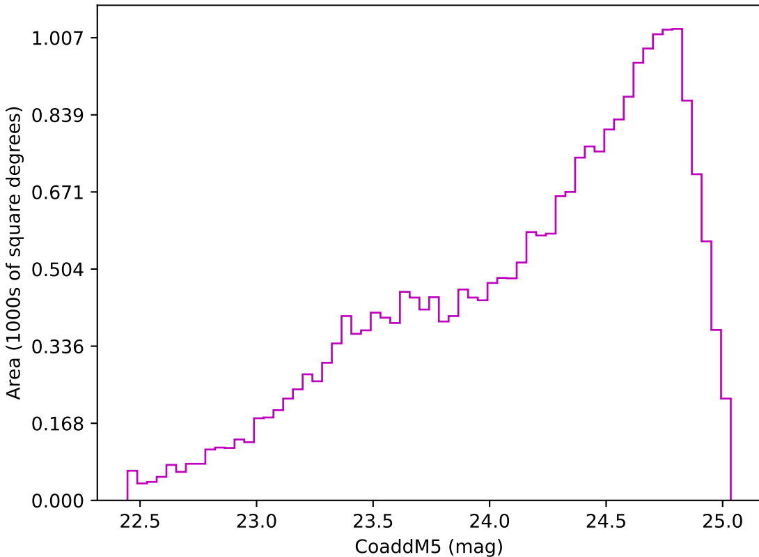
weather_cloudso0v3.4_10yrs Yr 3-4 z band: CoaddM5
