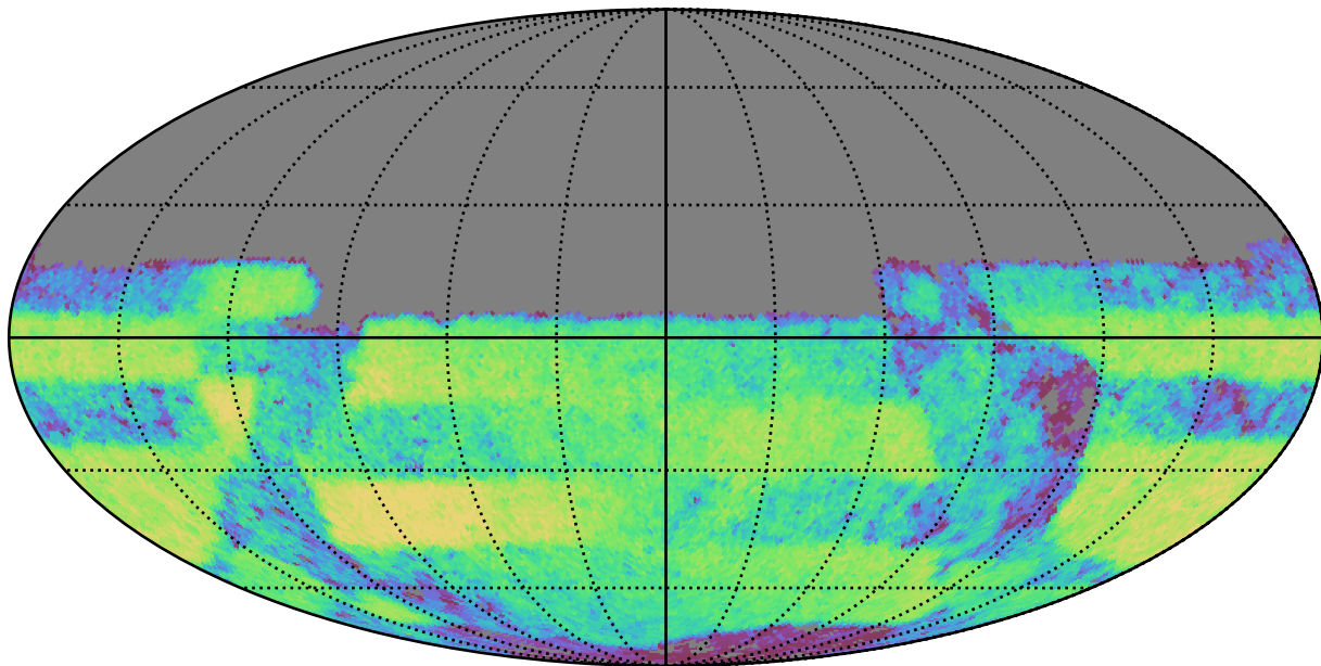
weather_cloudso0v3.4_10yrs Yr 3-4 y band: CoaddM5
