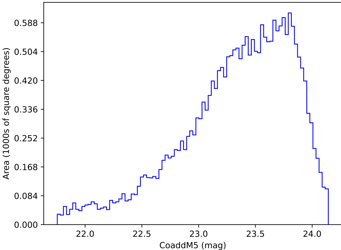
weather_cloudso0v3.4_10yrs Yr 3-4 y band: CoaddM5
