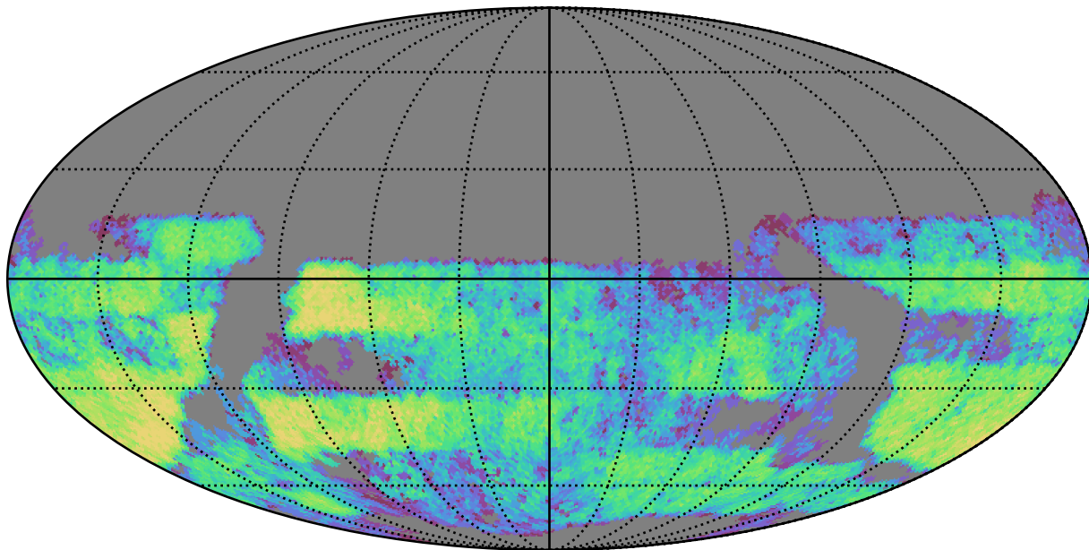
weather_cloudso0v3.4_10yrs Yr 3-4 u band: CoaddM5
