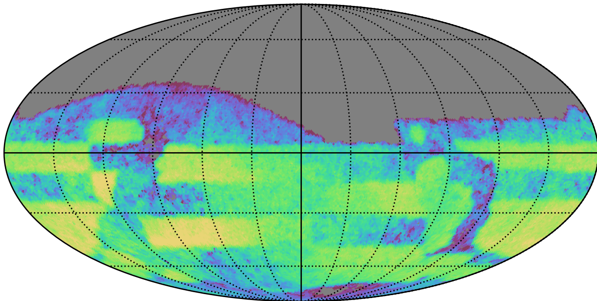
weather_cloudso0v3.4_10yrs Yr 3-4 r band: CoaddM5
