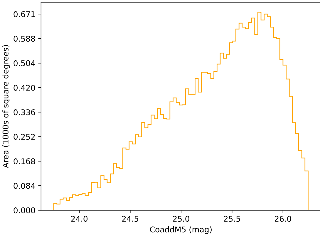
weather_cloudso0v3.4_10yrs Yr 3-4 r band: CoaddM5
