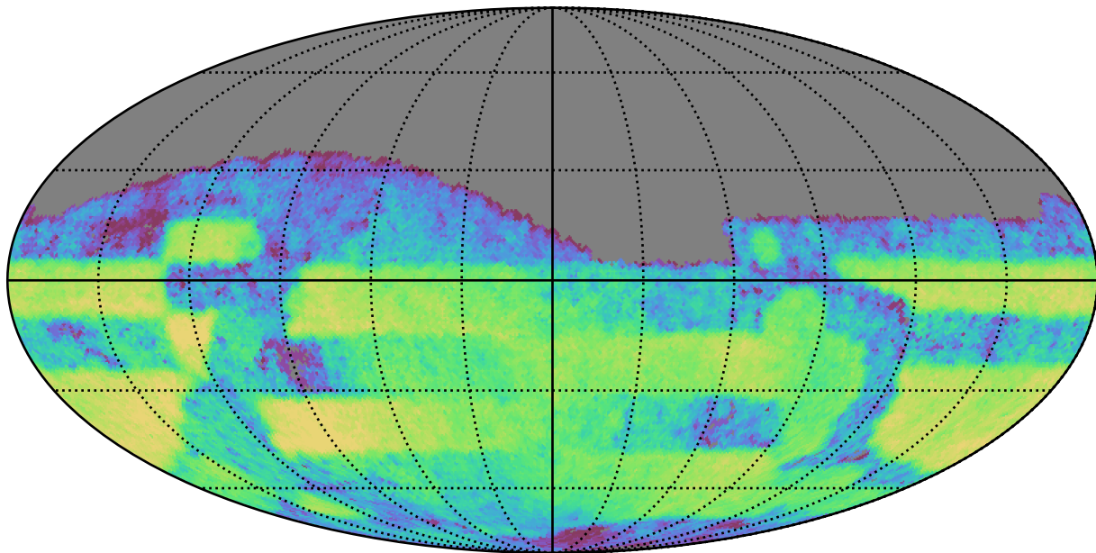
weather_cloudso0v3.4_10yrs Yr 3-4 i band: CoaddM5
