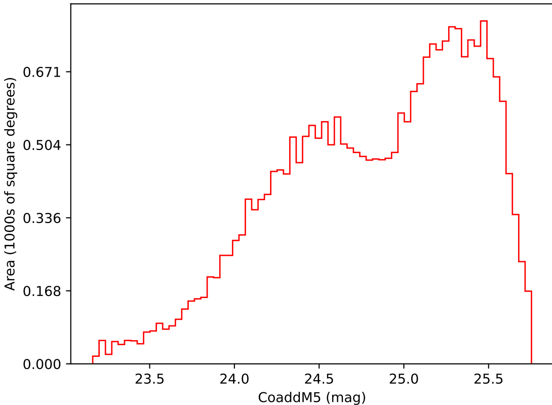
weather_cloudso0v3.4_10yrs Yr 3-4 i band: CoaddM5
