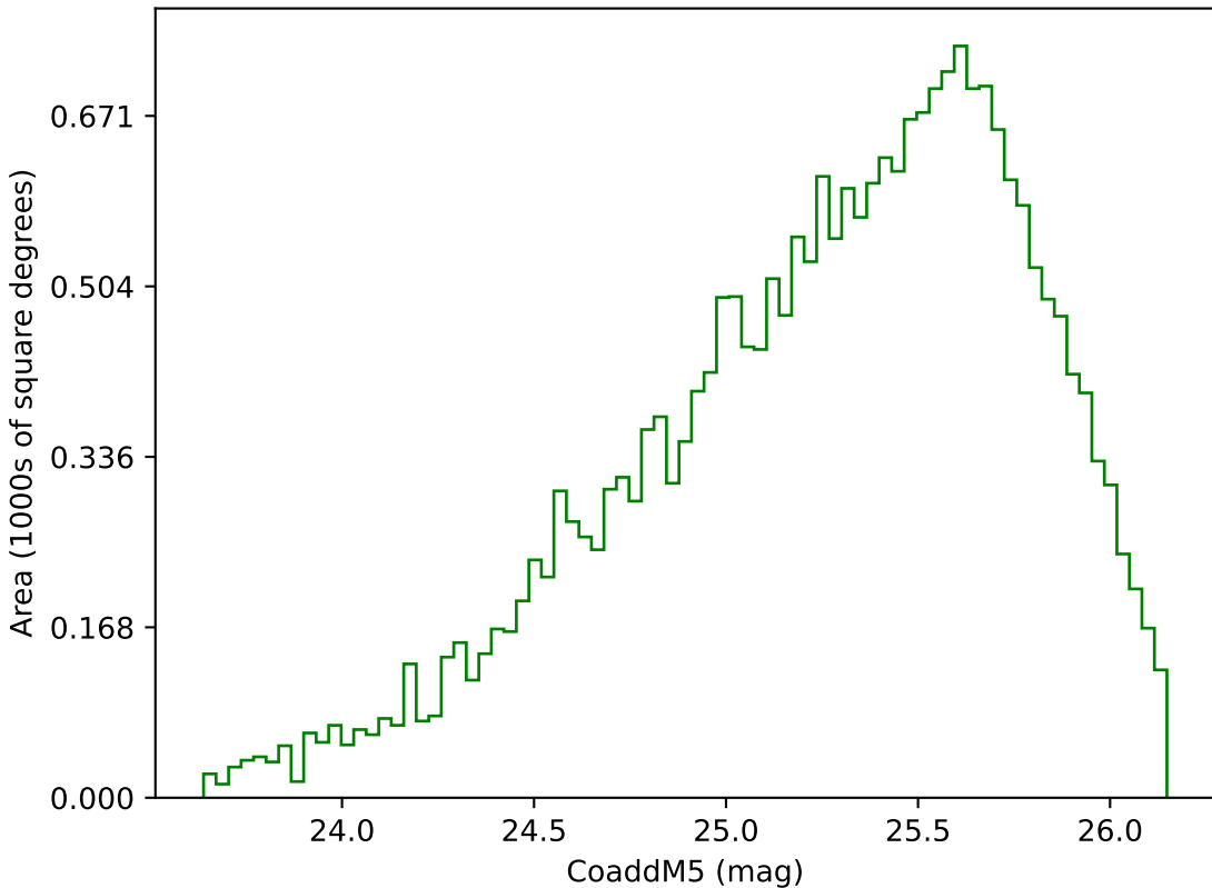
weather_cloudso0v3.4_10yrs Yr 3-4 g band: CoaddM5
