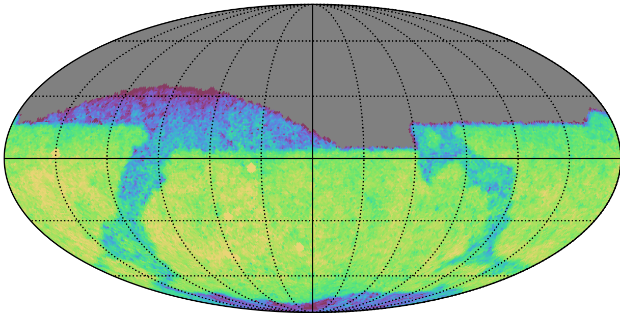
weather_cloudso0v3.4_10yrs Yr 1 z band: CoaddM5
