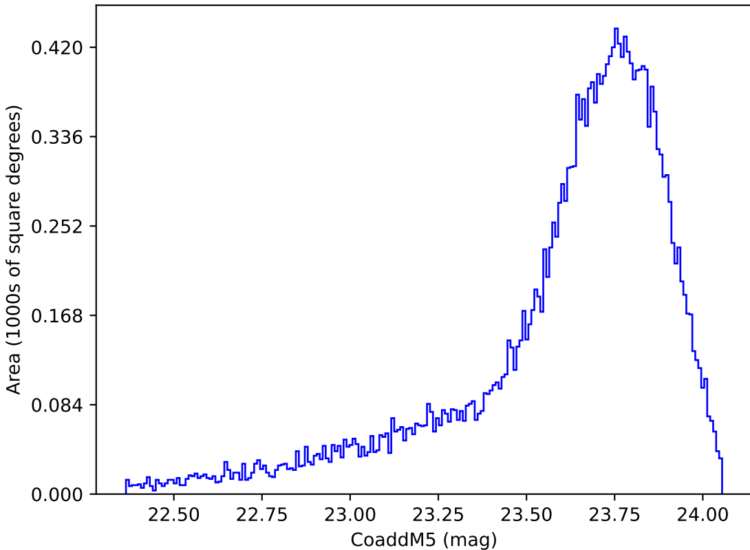
weather_cloudso0v3.4_10yrs Yr 1 y band: CoaddM5
