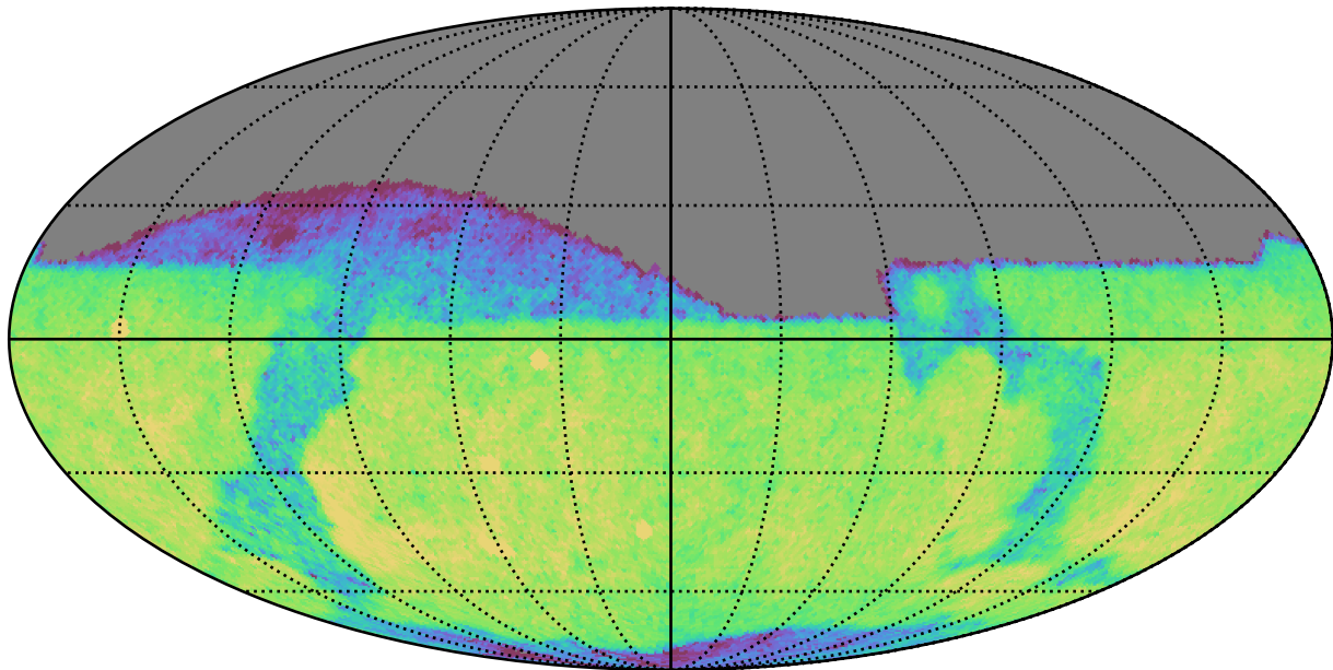
weather_cloudso0v3.4_10yrs Yr 1 r band: CoaddM5
