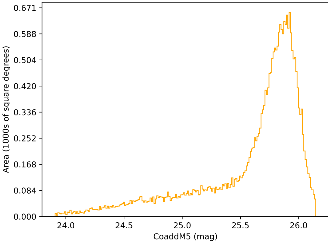
weather_cloudso0v3.4_10yrs Yr 1 r band: CoaddM5
