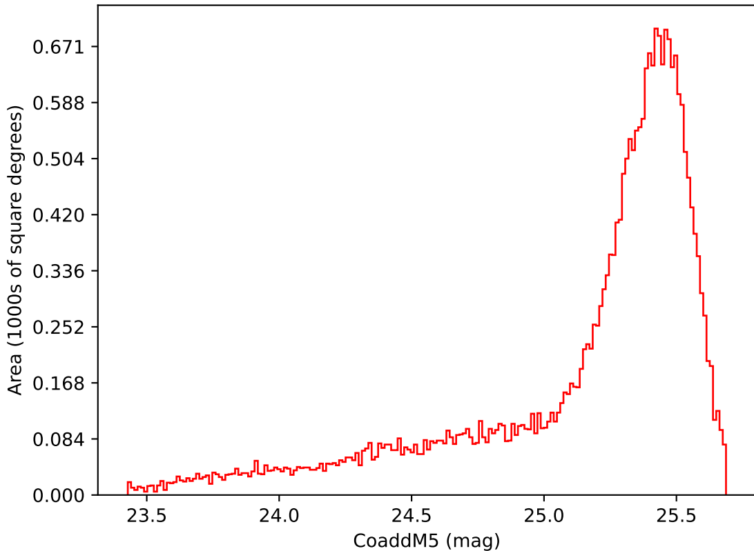
weather_cloudso0v3.4_10yrs Yr 1 i band: CoaddM5
