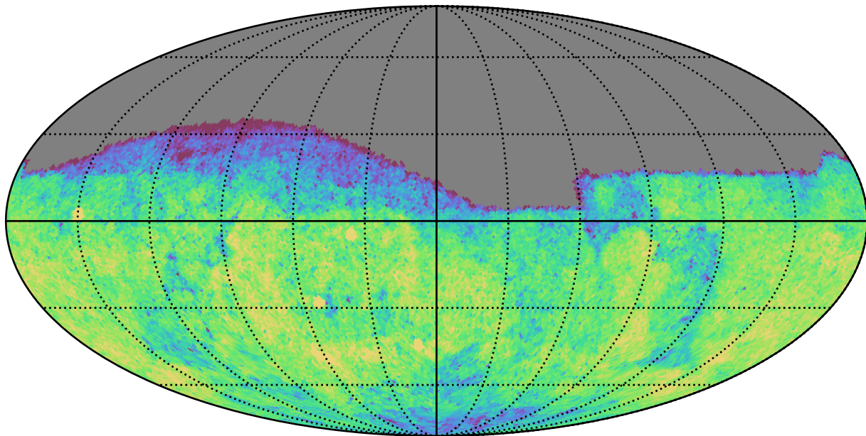
weather_cloudso0v3.4_10yrs Yr 1 g band: CoaddM5
