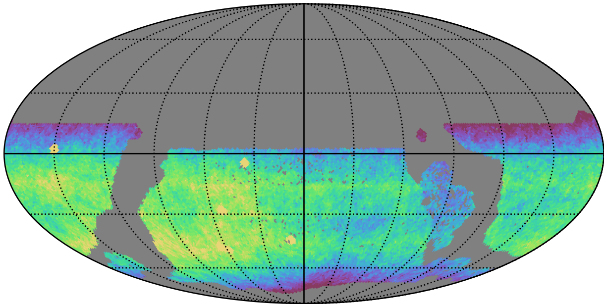
weather_cloudso0v3.4_10yrs WFD z band: CoaddM5
