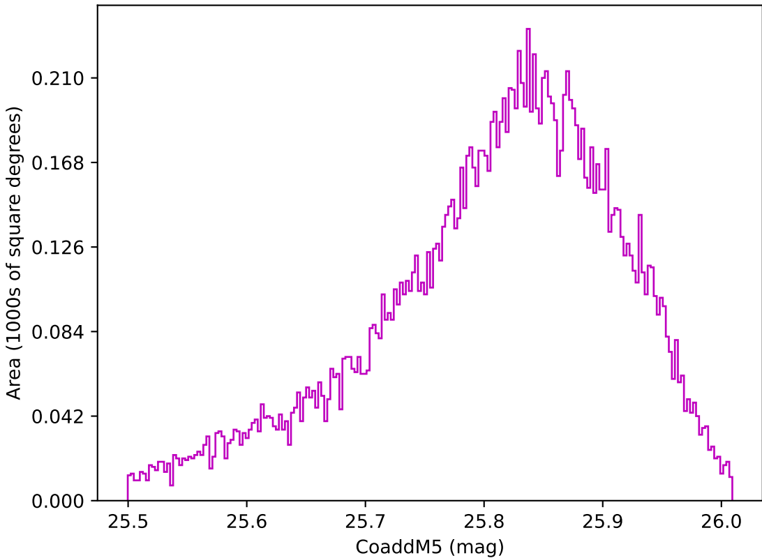
weather_cloudso0v3.4_10yrs WFD z band: CoaddM5
