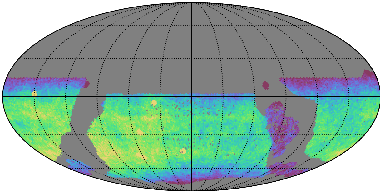
weather_cloudso0v3.4_10yrs WFD y band: CoaddM5
