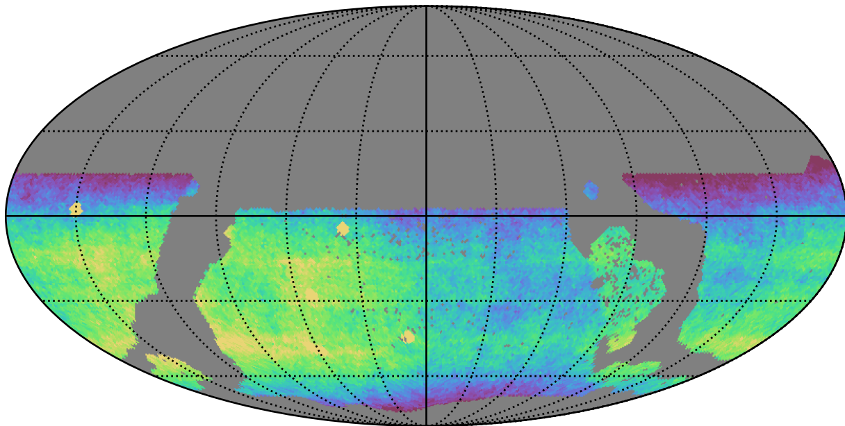
weather_cloudso0v3.4_10yrs WFD r band: CoaddM5
