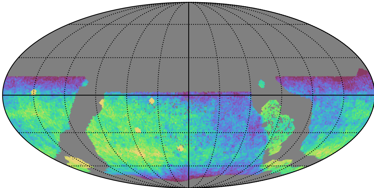
weather_cloudso0v3.4_10yrs WFD g band: CoaddM5
