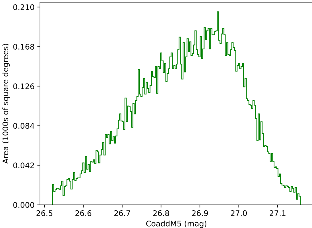
weather_cloudso0v3.4_10yrs WFD g band: CoaddM5
