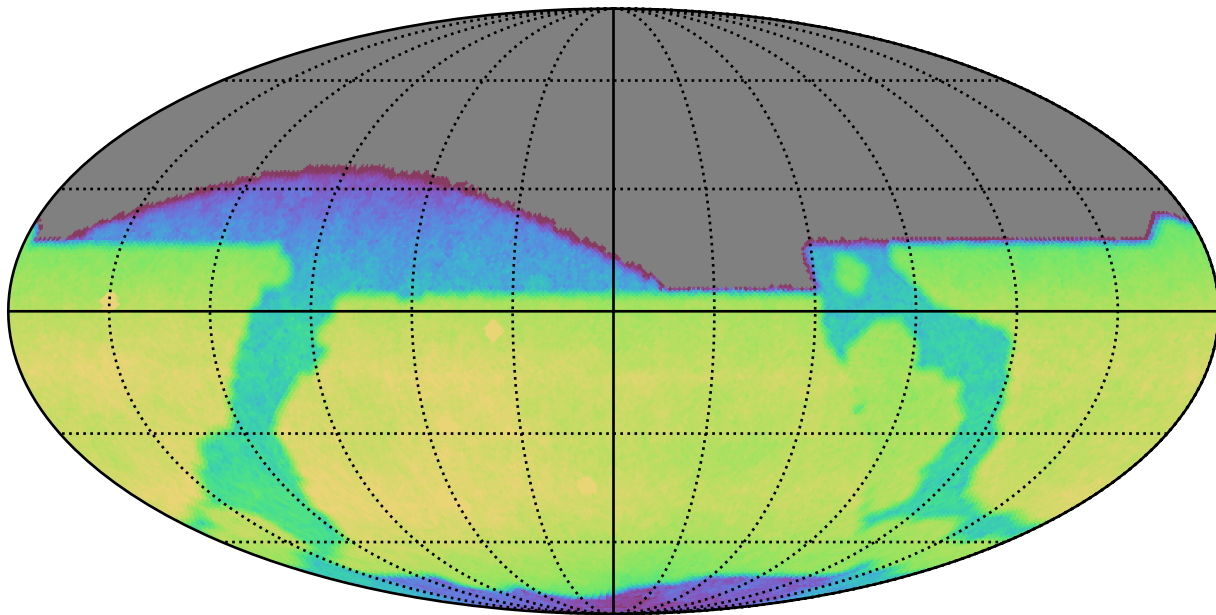
weather_cloudso0v3.4_10yrs All sky z band: CoaddM5
