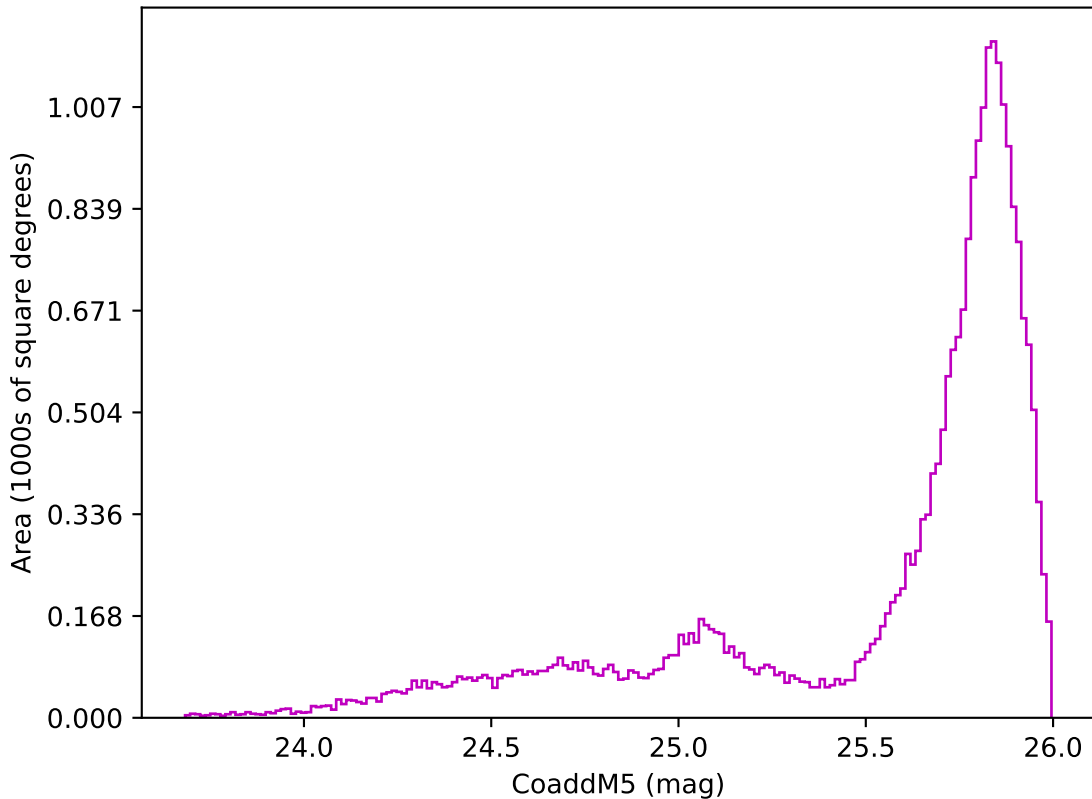
weather_cloudso0v3.4_10yrs All sky z band: CoaddM5
