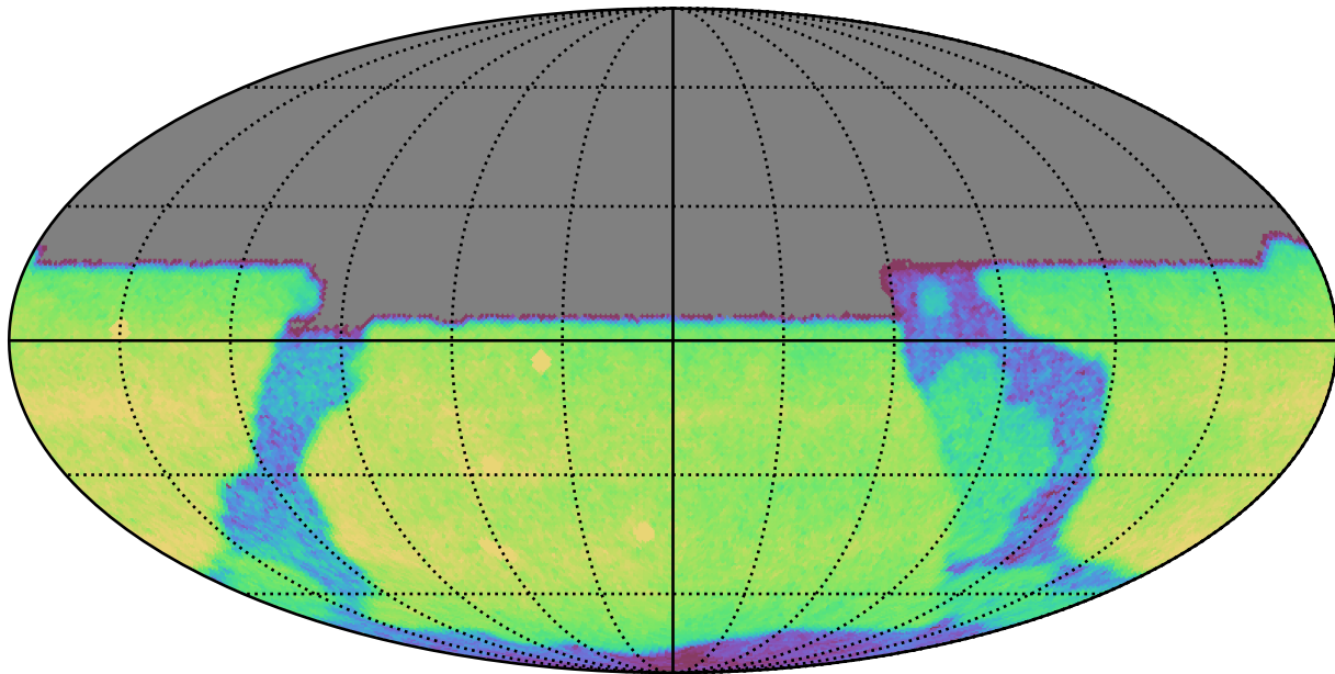
weather_cloudso0v3.4_10yrs All sky u band: CoaddM5
