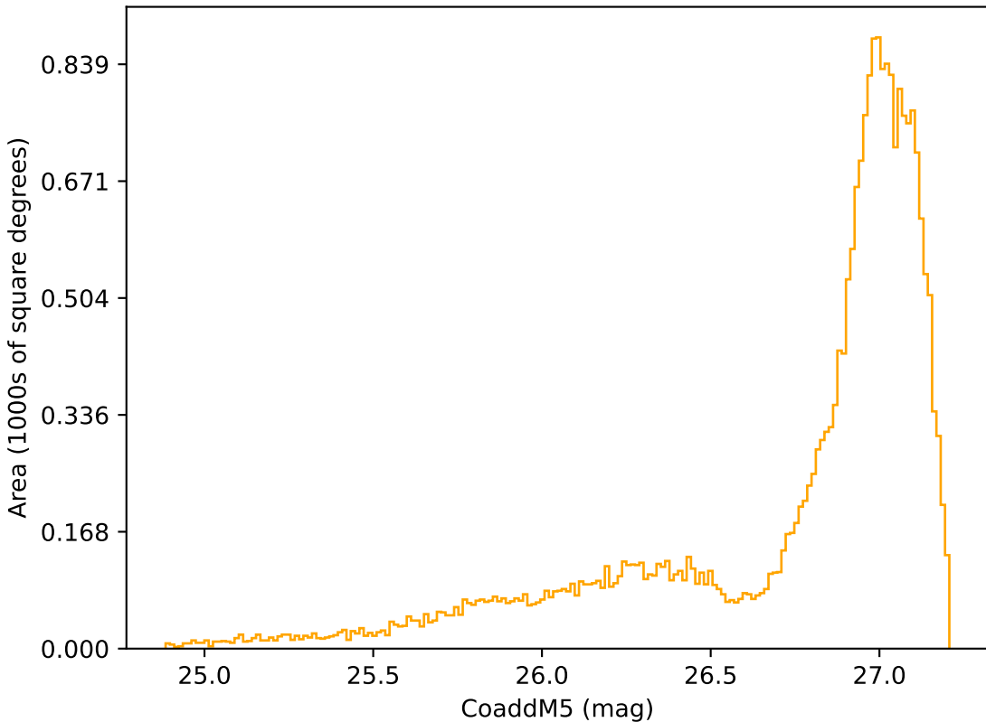
weather_cloudso0v3.4_10yrs All sky r band: CoaddM5
