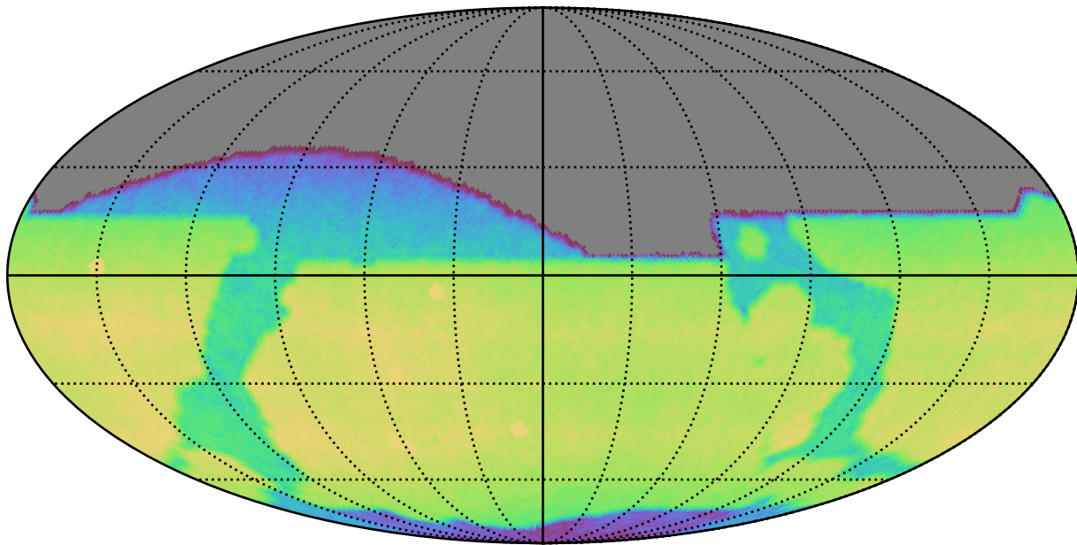
weather_cloudso0v3.4_10yrs All sky i band: CoaddM5
