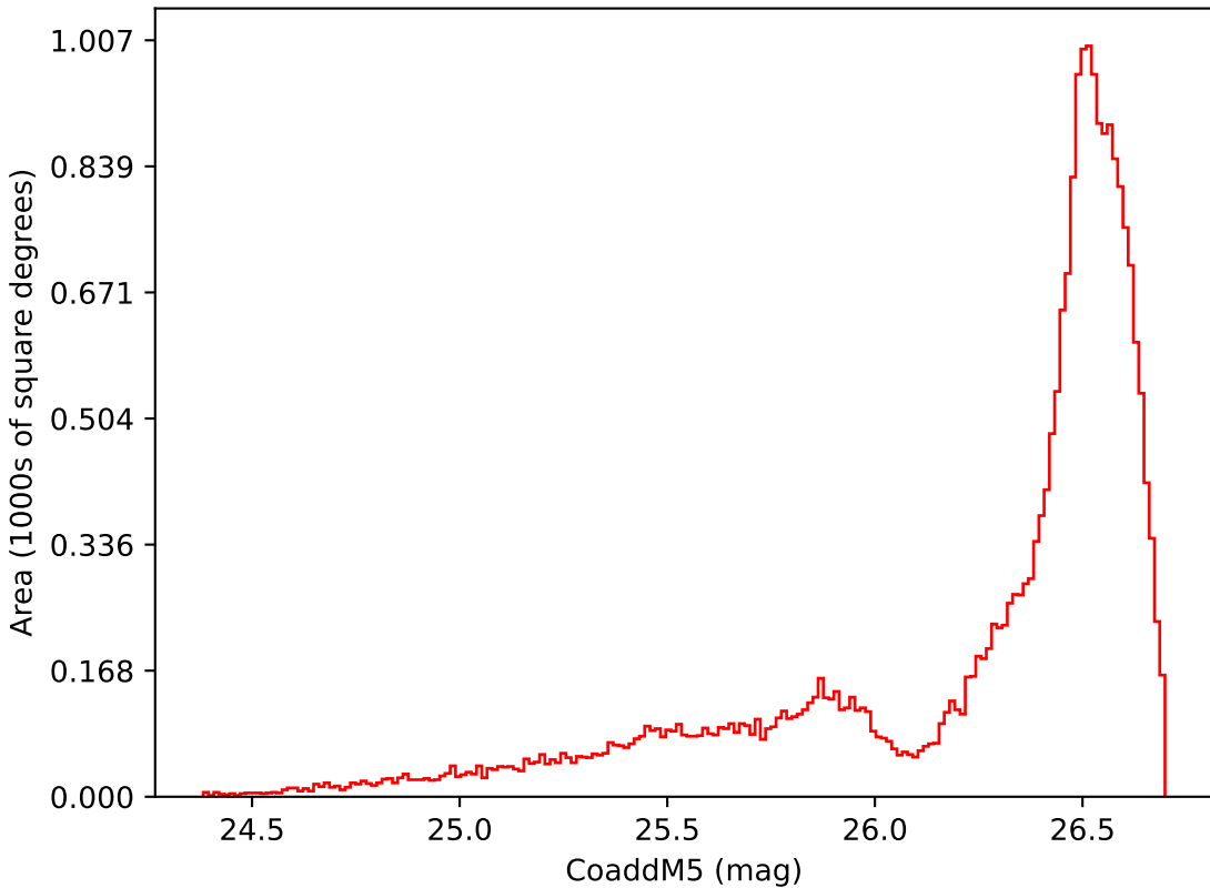
weather_cloudso0v3.4_10yrs All sky i band: CoaddM5
