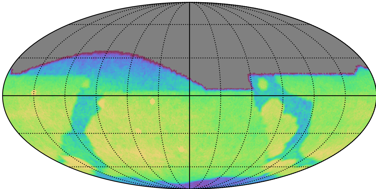
weather_cloudso0v3.4_10yrs All sky g band: CoaddM5
