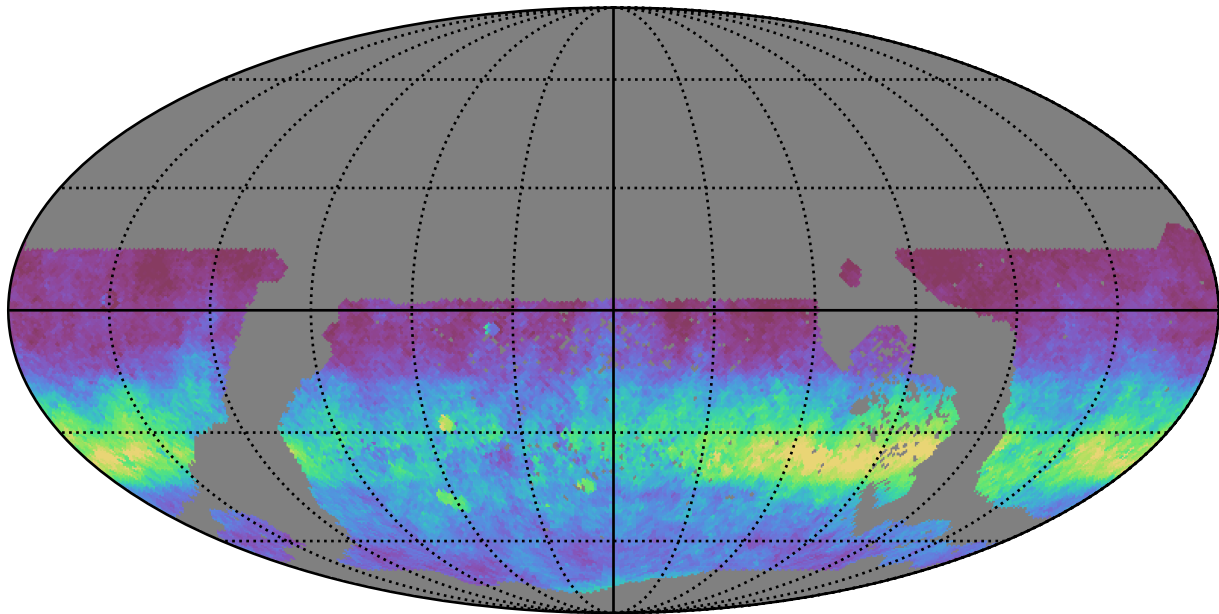
weather_cloudso0v3.4_10yrs WFD r band: AngleRms rotSkyPos
