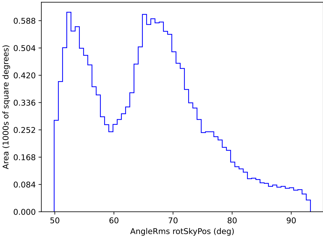
weather_cloudso0v3.4_10yrs WFD all bands: AngleRms rotSkyPos
