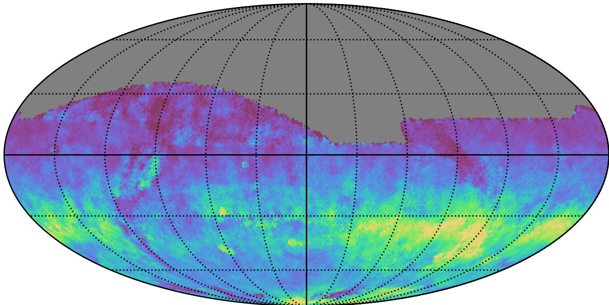
weather_cloudso0v3.4_10yrs All sky z band: AngleRms rotSkyPos
