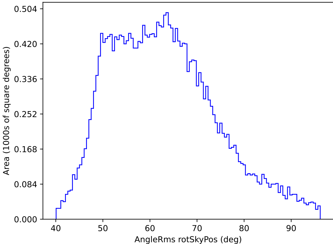
weather_cloudso0v3.4_10yrs All sky z band: AngleRms rotSkyPos
