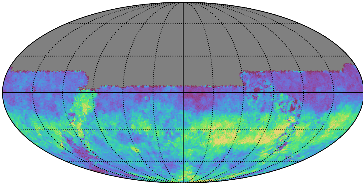
weather_cloudso0v3.4_10yrs All sky u band: AngleRms rotSkyPos
